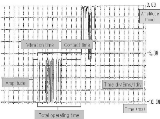
Fig. 11 Experimental results by using system analyzer
